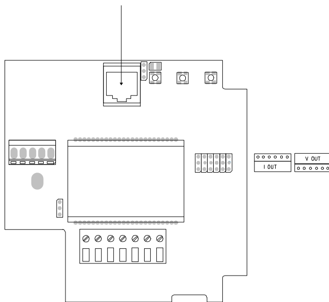
Figure 2 Calibration Connector X5 in Series HMP230 Transmitters
