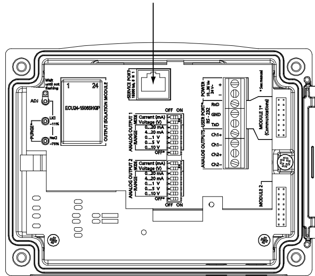
Figure 4 Service Port in Series HMT330 Transmitters
