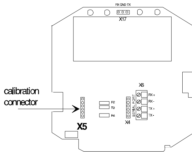
Figure 2 Calibration Connector X5 in Series HMP230 Transmitters
